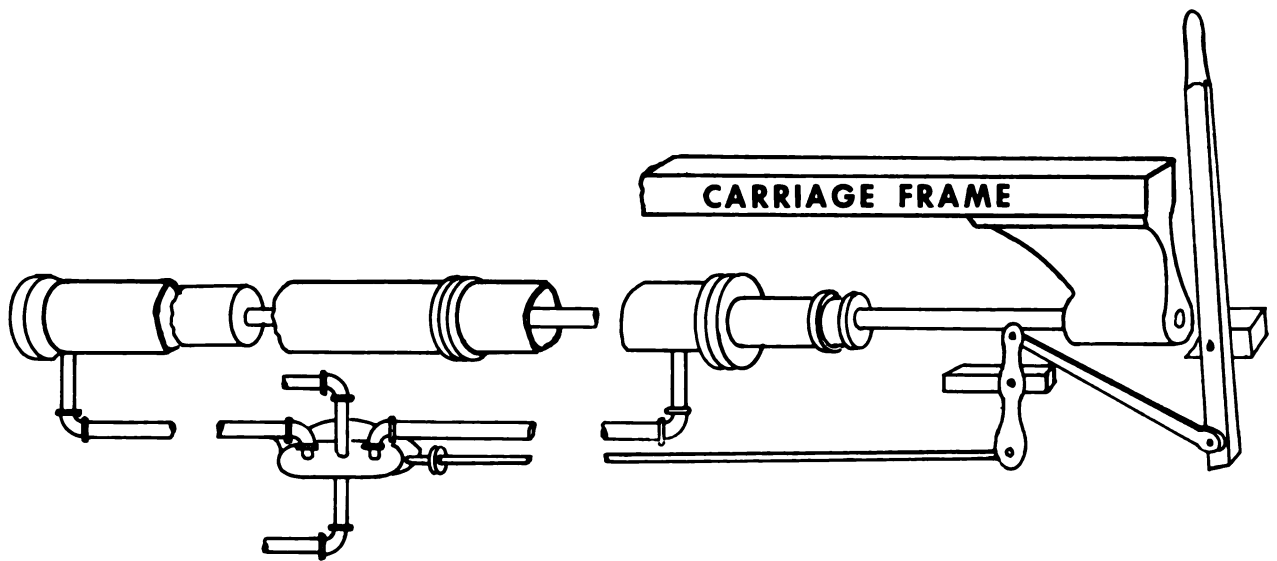
Figure 8-11. Single-cylinder steam piston feed works.
